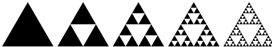
Figure 3.10: Evolution of the Sierpinski triangle
