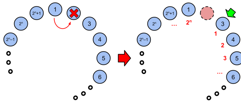
Figure 2.8: Illustration of the Josephus Problem with a different number of players.
